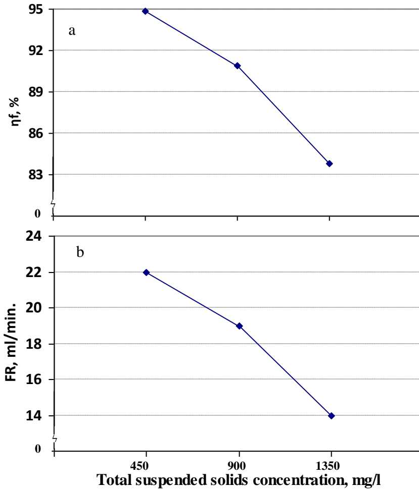
Fig. (2) Effect of total suspended solids concentration, mg/l on (ηf), % (a) and (FR), ml/min (b).
