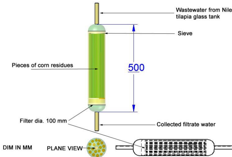
Fig. 1a: Corn stems filter.
