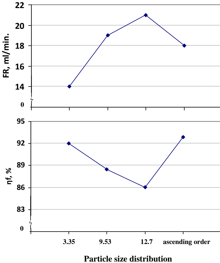
Fig. (3) Effect of residues, mm on ( \eta_f ), % and (FR), ml/min.
