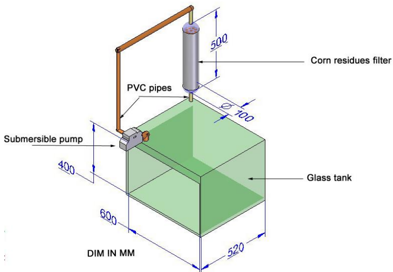
Fig. 1 b Designed filtration system
