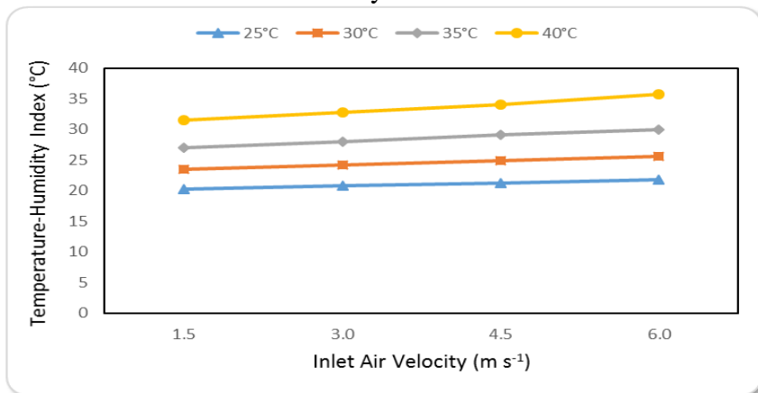
Figure (15): The temperature-humidity index effectiveness at different ambient temperatures and inlet air velocities.
