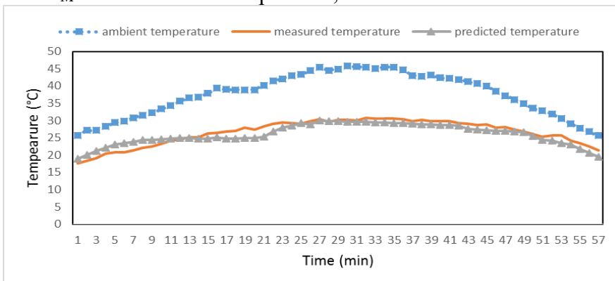
Figure (18): The predicted and the measured outlet temperatures of evaporative cooling system.
