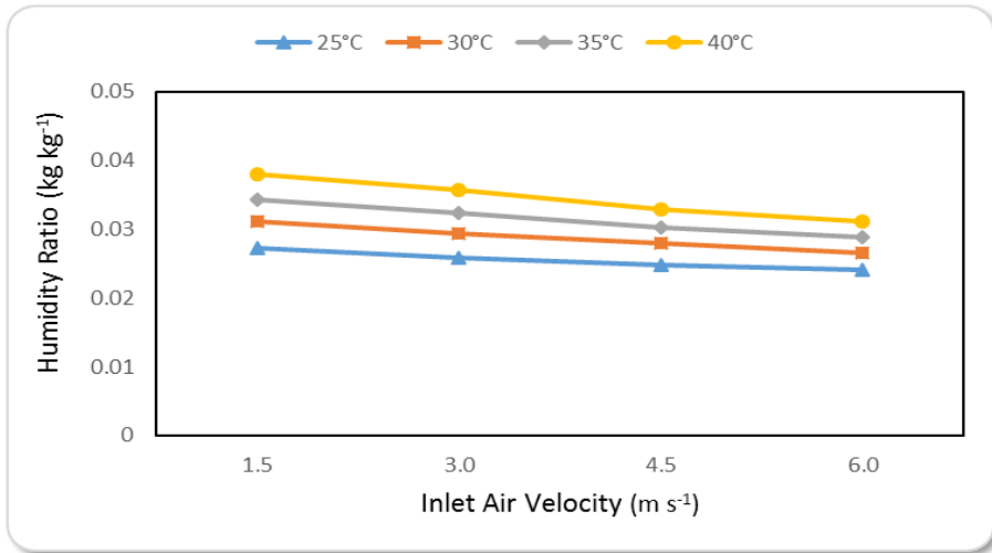
Figure (12): The humidity ratio effectiveness at different ambient temperatures and inlet air velocities.
