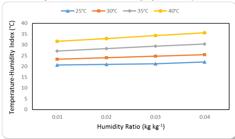
Figure (16): The temperature-humidity index effectiveness at different ambient temperatures and humidity ratios.
