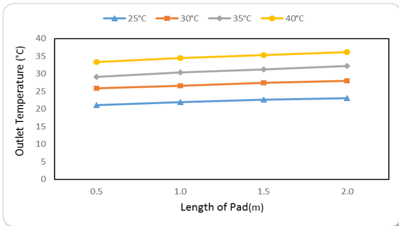
Figure (5): The outlet temperature at different ambient temperatures and lengths of pad.
