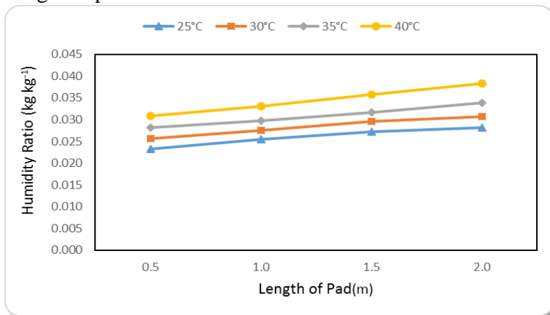
Figure (14): The humidity ratio effectiveness at different ambient temperatures and lengths of pad.
