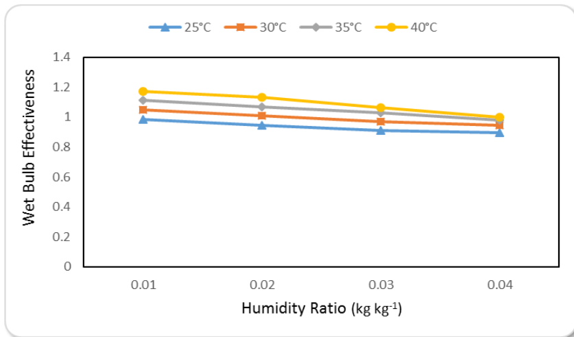
Figure (7): The wet bulb effectiveness at different ambient temperatures and humidity ratios.
