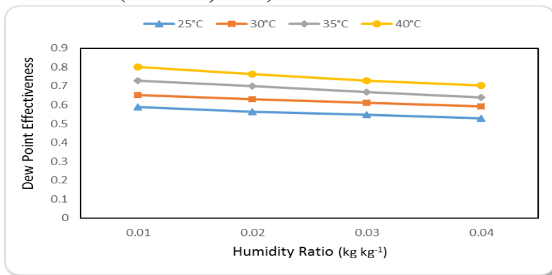
Figure (10): The dew point effectiveness at different ambient temperatures and humidity ratios.
