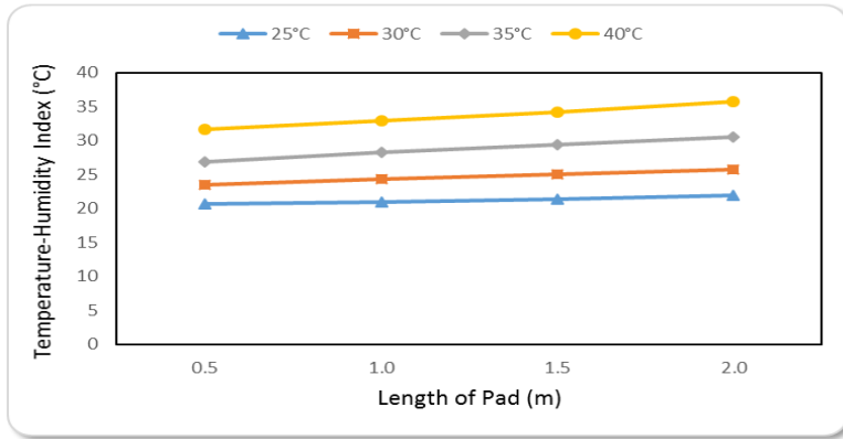
Figure (17): The temperature-humidity index effectiveness at different ambient temperatures and lengths of pad.
