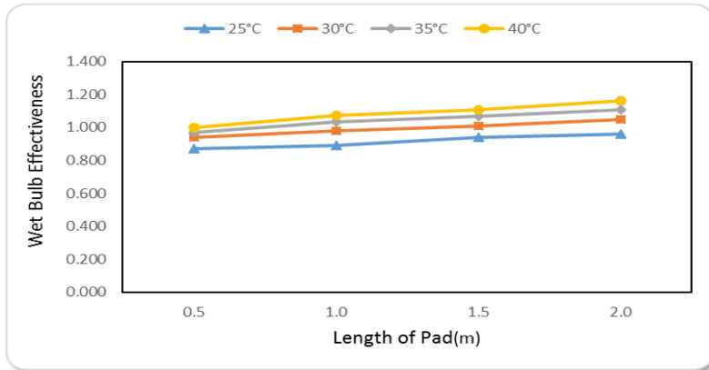
Figure (8): The wet bulb effectiveness at different ambient temperatures and lengths of pad.
