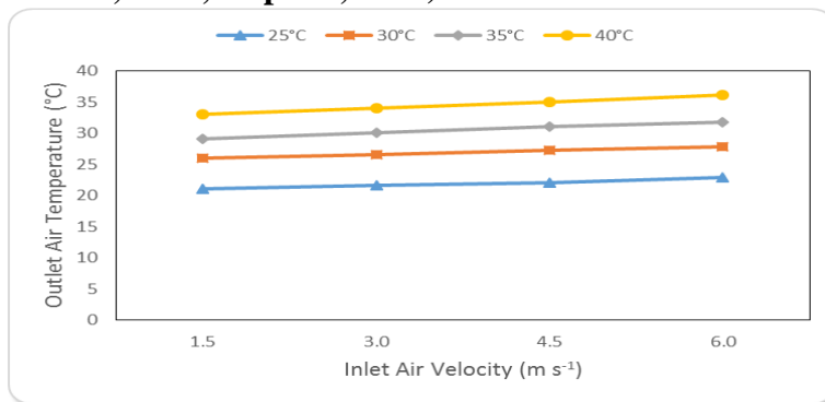
Figure (3): The outlet temperature at different ambient temperatures and inlet air velocities for the direct evaporative cooling system.
