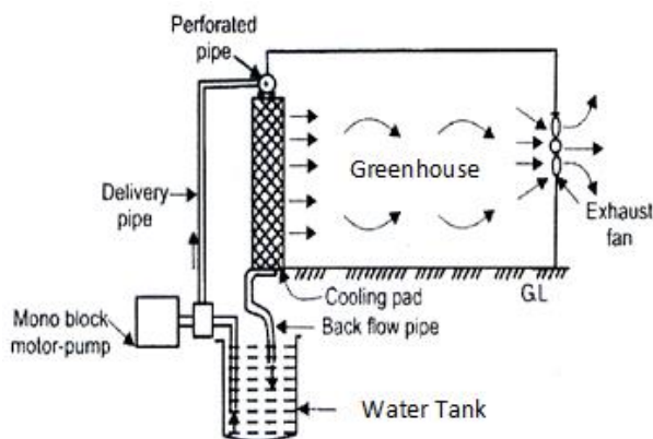
Figure (2): Evaporative cooling system components.
