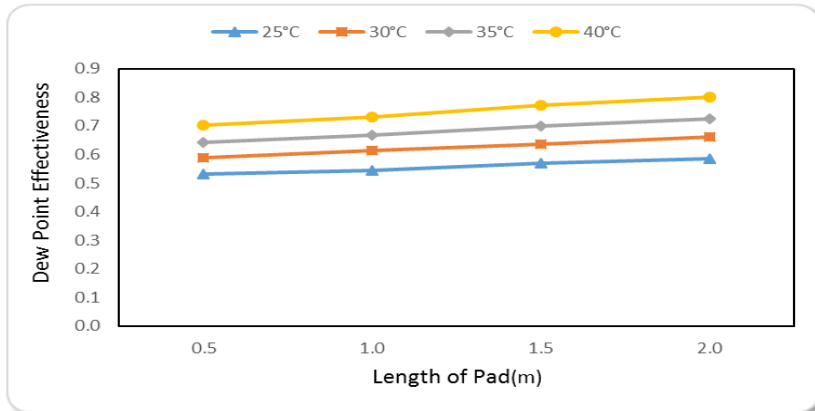
Figure (11): The dew point effectiveness at different ambient temperatures and lengths of pad.
