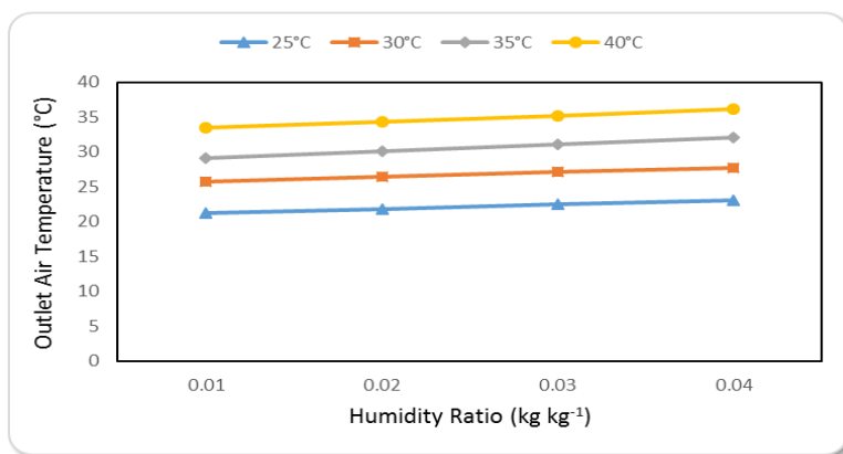
Figure (4): The outlet temperature at different ambient temperatures and humidity ratios.
