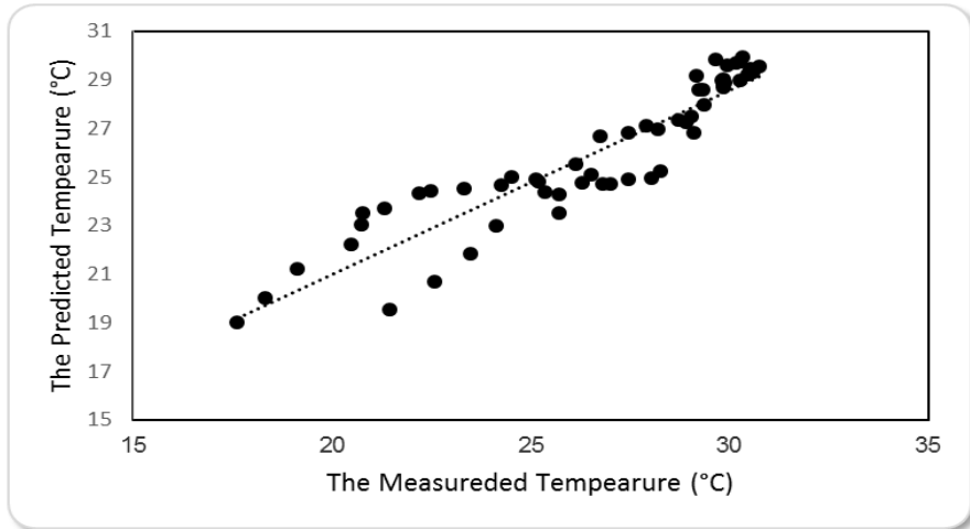
Figure (19): The comparison between the predicted and the measured outlet temperatures of evaporative cooling system.
