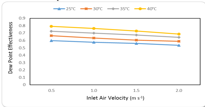
Figure (9): The dew point effectiveness at different ambient temperatures and inlet air velocities.
