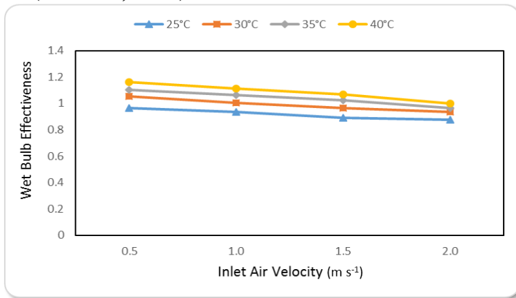
Figure (6): The wet bulb effectiveness at different ambient temperatures and inlet air velocities.
