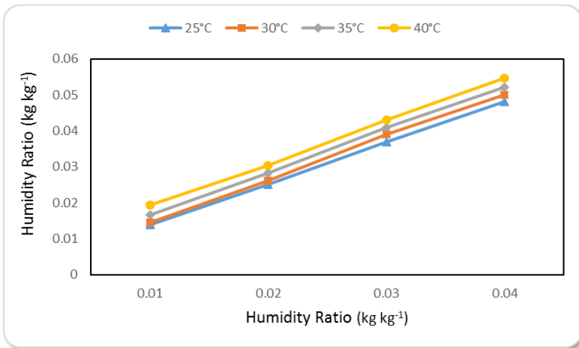
Figure (13): The humidity ratio effectiveness at different ambient temperatures and humidity ratios.
