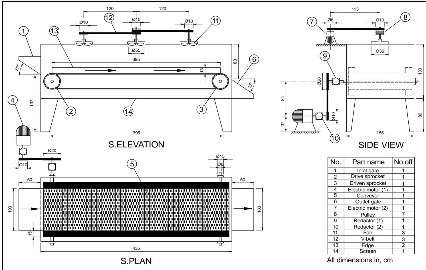
Fig. (1): The schematic drawing of the manufactured single-pass feed pellets cooler.
