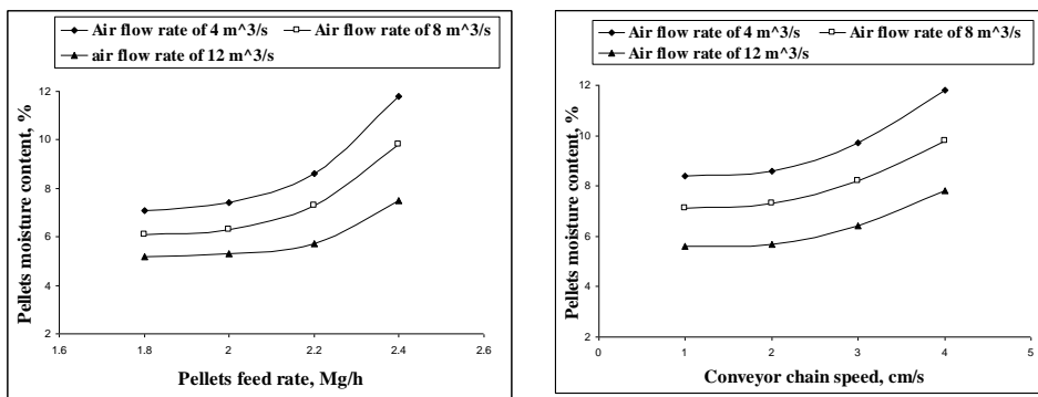
Fig. (2): Effect of pellets feed rate, conveyor chain speed and air flow rate on pellets moisture content
