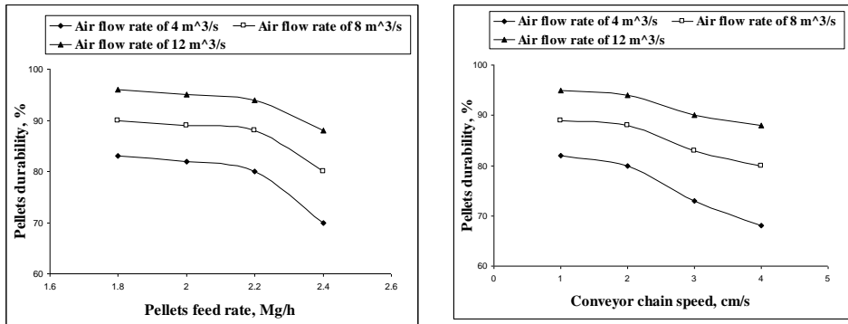
Fig. (4): Effect of pellets feed rate, conveyor chain speed and air flow rate on pellets durability
