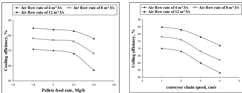
Fig. (3): Effect of pellets feed rate and conveyor chain speed on cooling efficiency under different air flow rates
