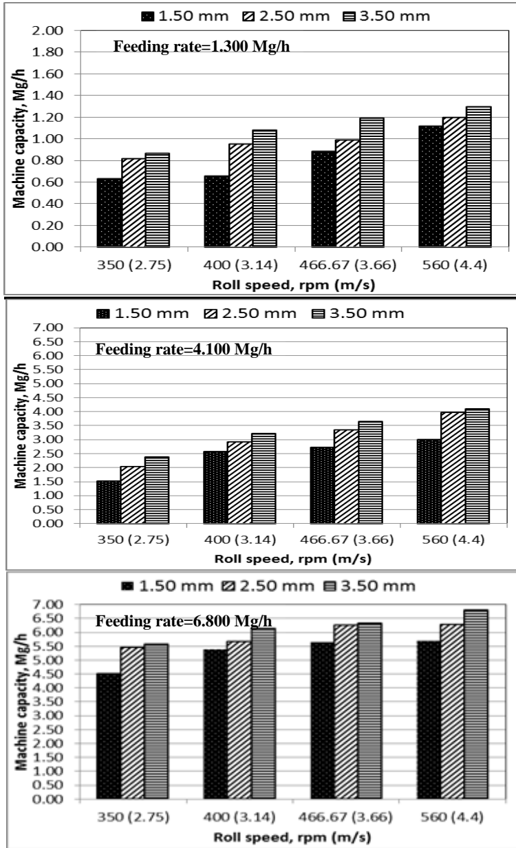
Fig.(6): Effect of rolls speed and feeding rate on the machine capacity using different roll clearances.
