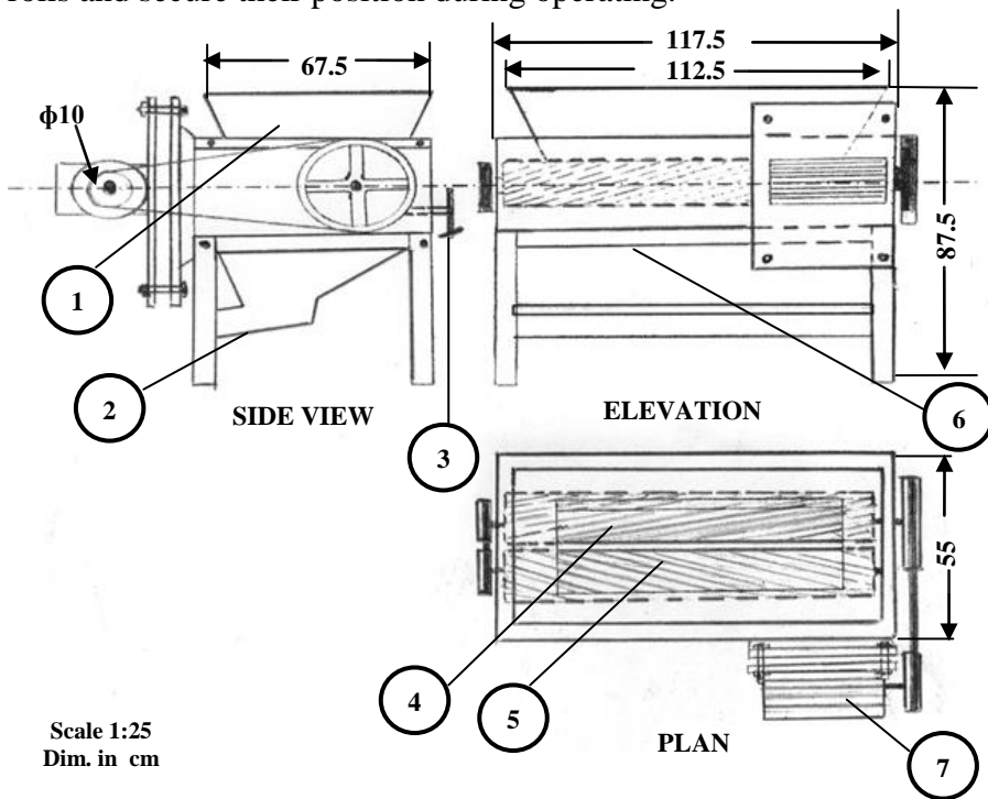
(1) Feed hopper, (2) Outlet chute, (3) roll clearance adjustment screw, (4) Drive roll, (5) Driven roll, (6) Frame, (7) Electric motor.
