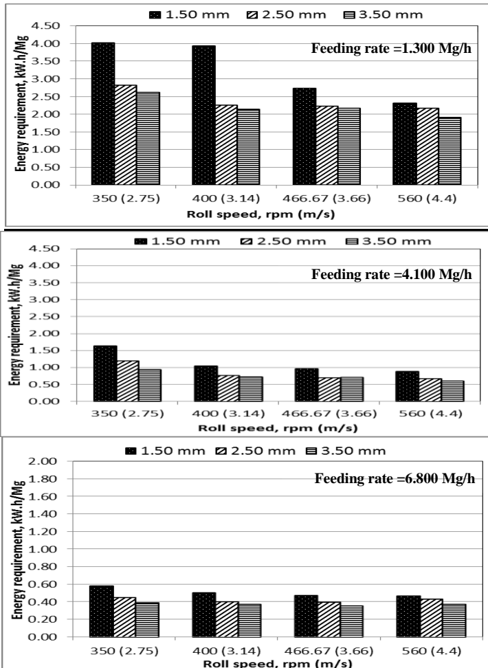
Fig.(8): Effect of rolls speed and feeding rate on the energy requirement under different roll clearances
