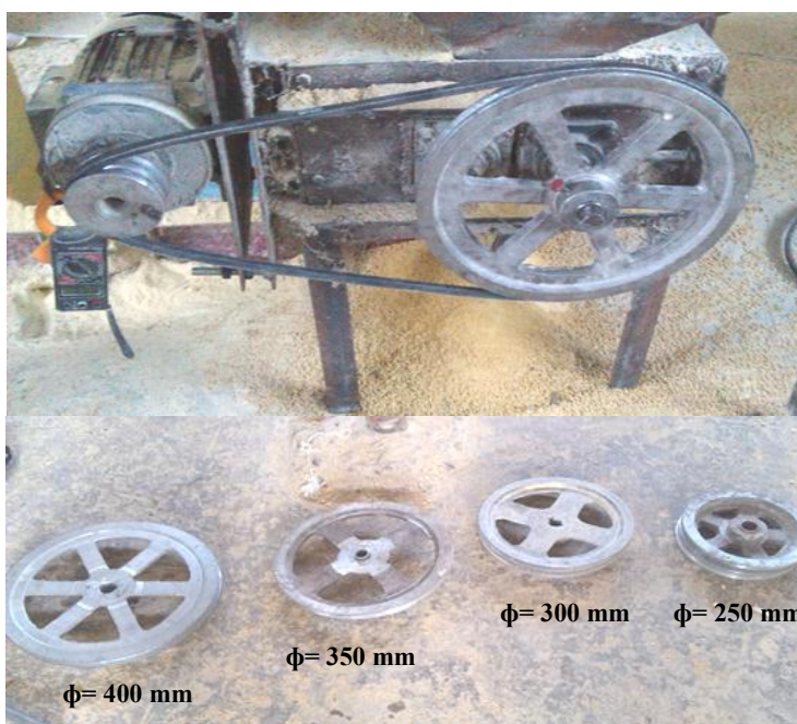
Fig.(4): The transmission unit using different pulley's diameters.
