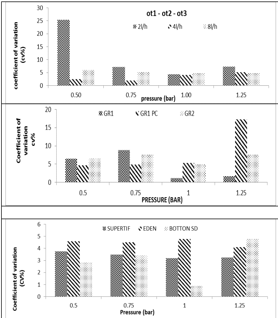
Fig 4: Manufacture coefficient of variation (CV %), for the tested drippers under different operating pressure (bar).
