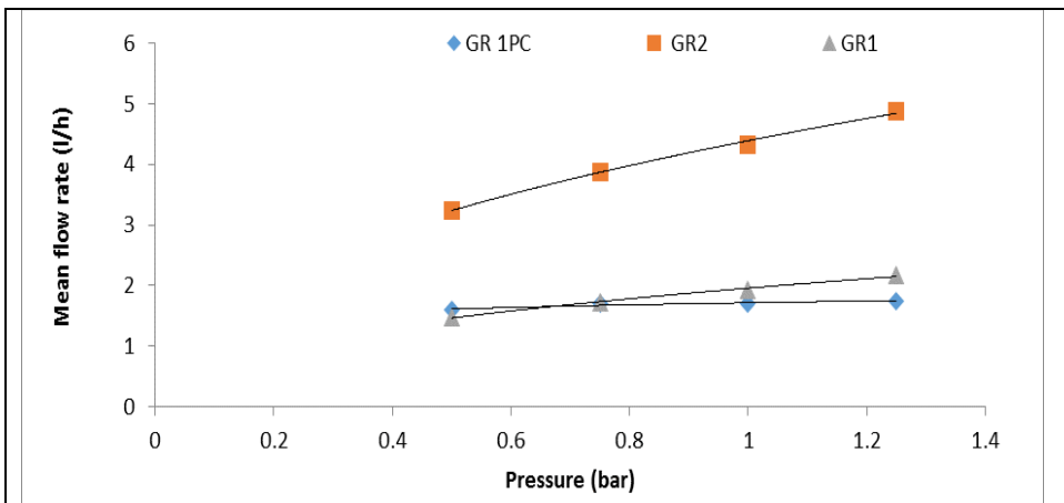
Fig 3: Performance curves of the acceptable tested dripper types.
