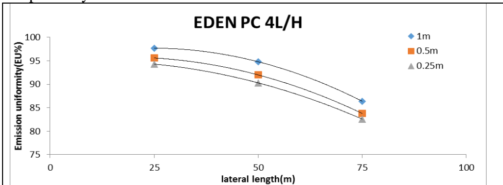
Fig (7) Effect of lateral length on Emission uniformity under different dripper spacing (0.25-0.50-1m)for 4L/h PC.
