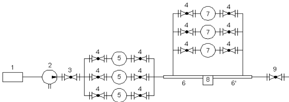
Fig (2) General sketch showing pressure drop test facility.
