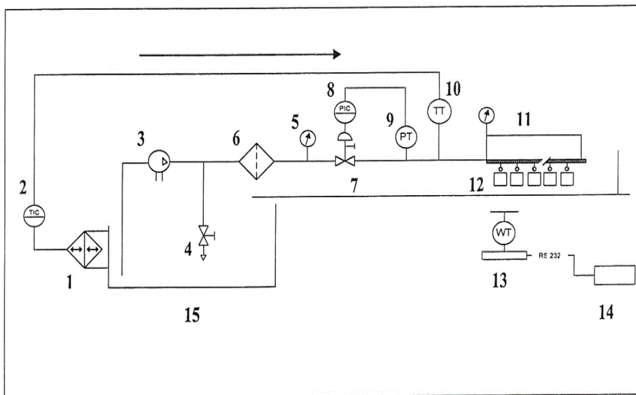
Fig. (1): Drip irrigation test facility.
