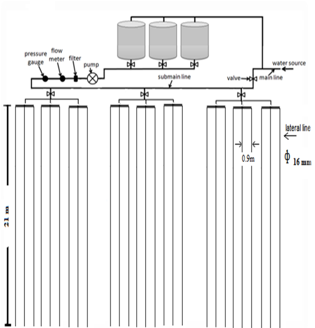
Fig. (2): The irrigation system components.
