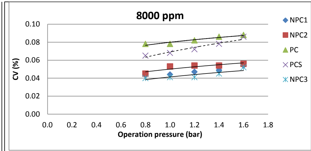
Fig. (5): The effect of emitter type on the coefficient of variation (CV) under different pressure head.
