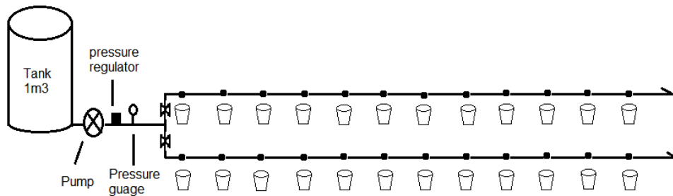
Fig. (1): Lab experiment layout.
