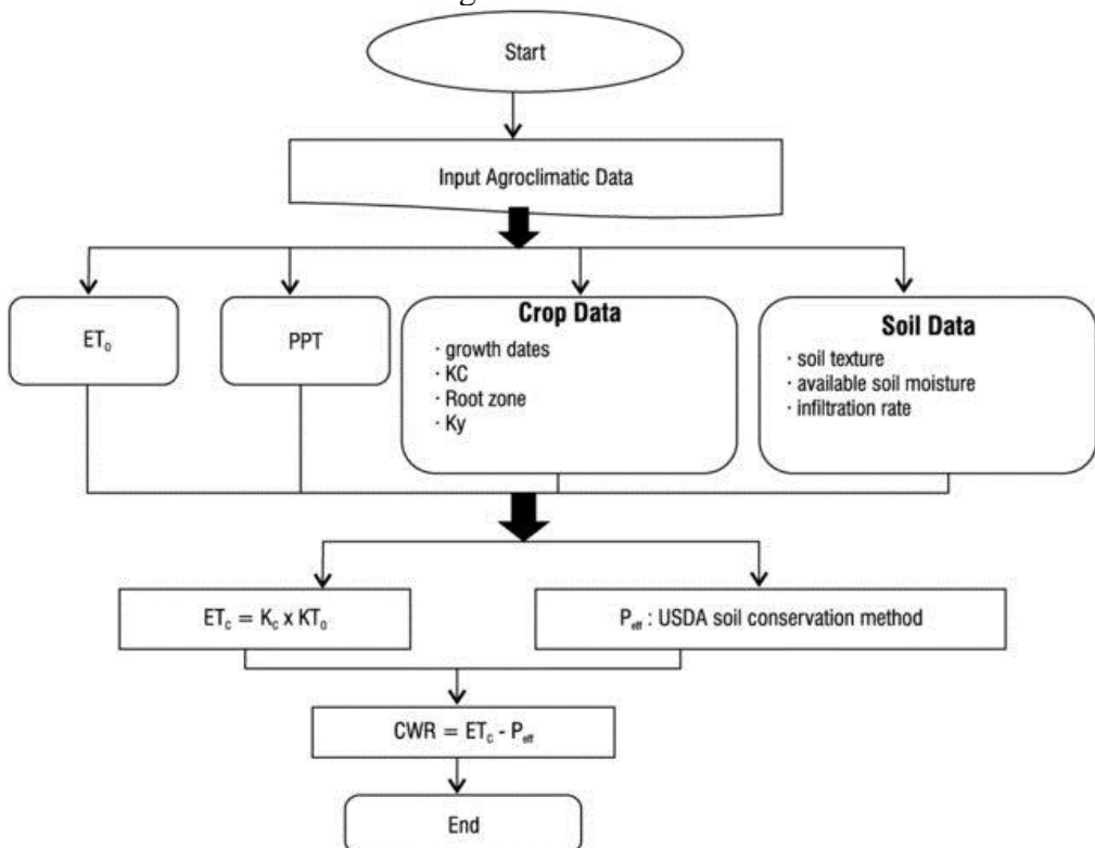
Figure 4: Flow chart of FAO-CROPWAT
