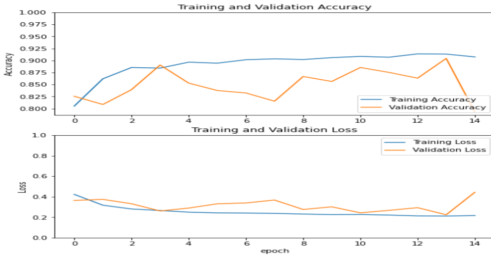
(a) Inception-v3
