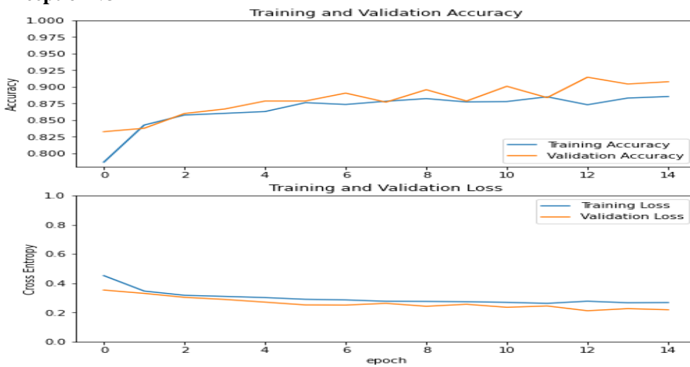
(b) Inception-ResNet-v2
