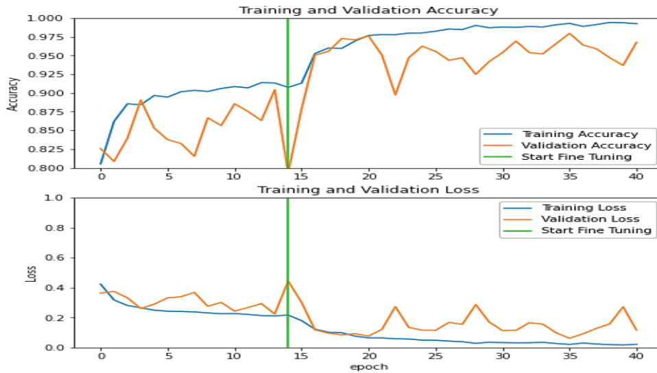
(a) Inception-v3
