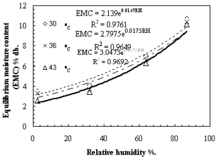
Fig (5) Adsorption isotherms for G5 variety at three different temperatures
