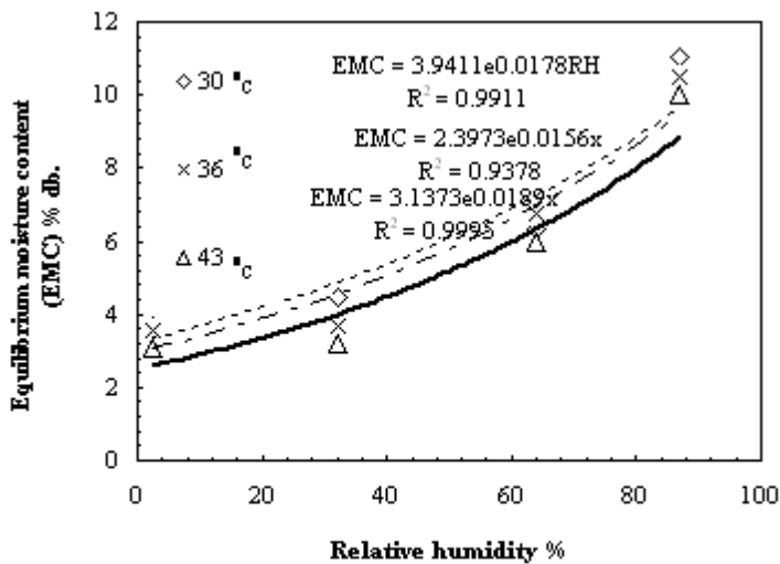
Fig(3) Desorption isotherms for G5 variety at three different temperatures.
