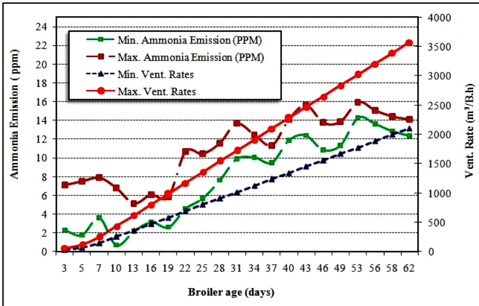
Fig. (3). Min. and maximum ammonia emission (ppm) in opposition to minimum and maximum ventilation rates (m³/B.h).
