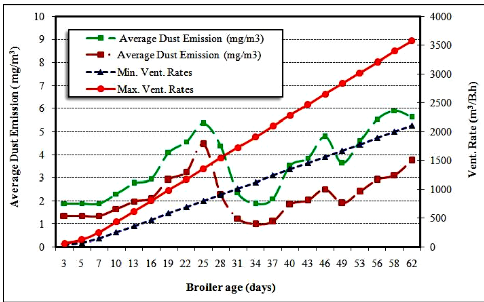
Fig. (4). Average dust emission rate ( \text{mg}/\text{m}^3 ) vs. minimum and maximum ventilation rates ( \text{m}^3/\text{B.h} ).
