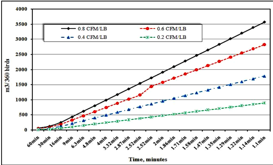
Fig.(1). Maximum ventilation rates 0.2, 0.4, 0.6 and 0.8 CFM/LB.
