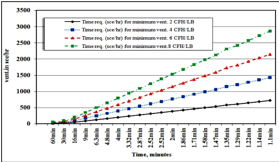
Fig. (2). Time required in seconds for every hour under minimum vent.
