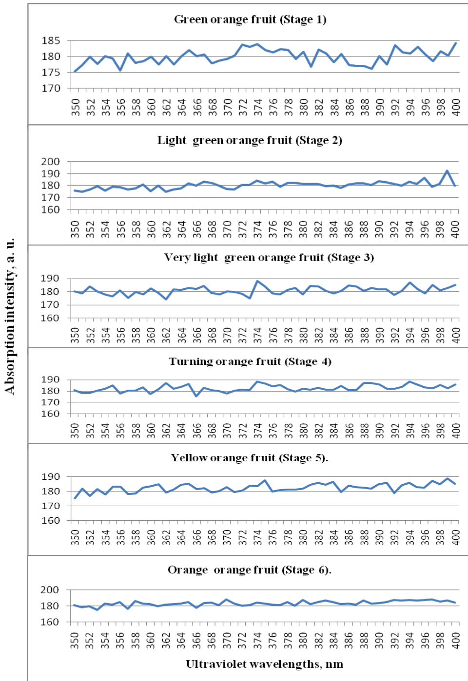
Fig. (3) : Absorption intensity of ultraviolet light from orange fruits at different maturity stages.
