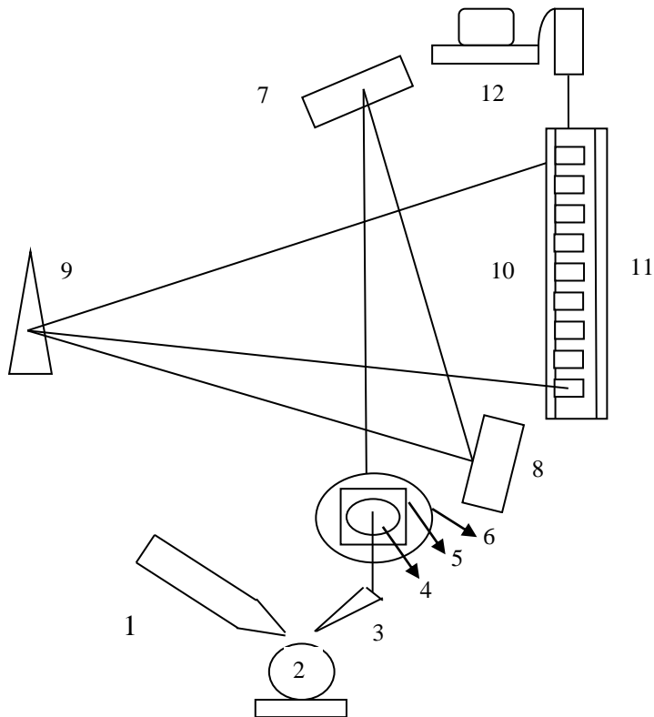
b) Diagram of spectrum setup
