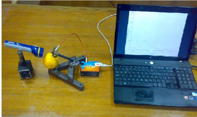
a) Photo of spectrum setup.
