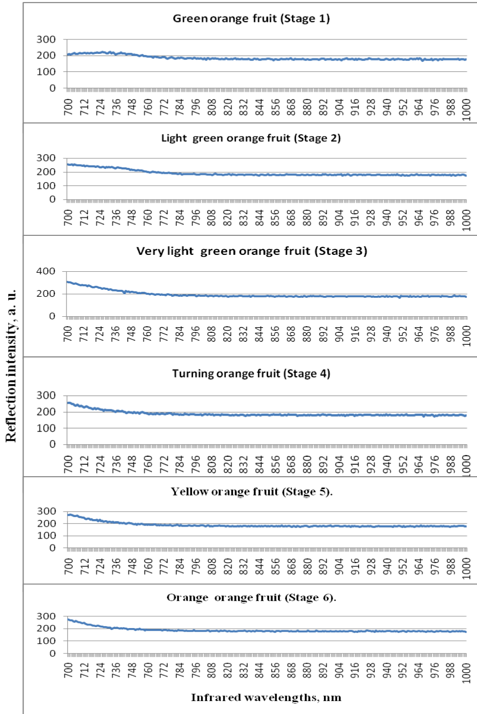
Fig. (4) : Reflection intensity of infrared light from orange fruits at different maturity stages.
