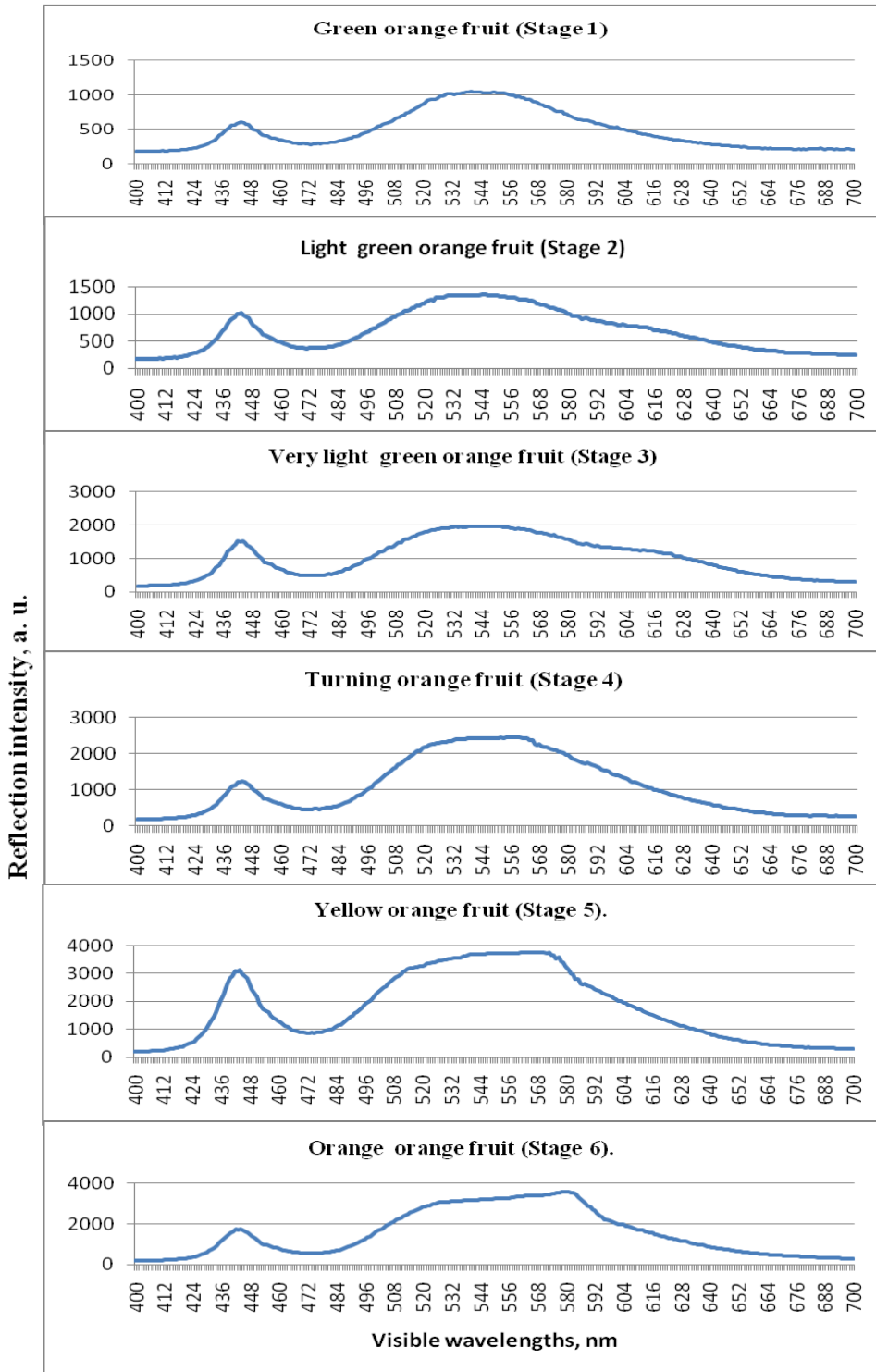
Fig. (6) : Reflection intensity of visible light from orange fruits at different maturity stages.
