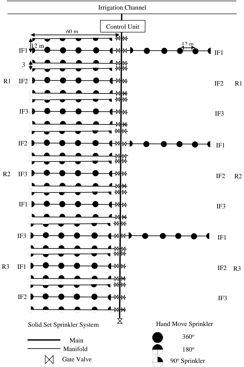
Figure 1. Experiment Layout
