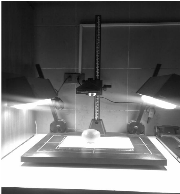
Fig. 1: Schematic diagram setup for measuring color properties of apple fruit defects.
