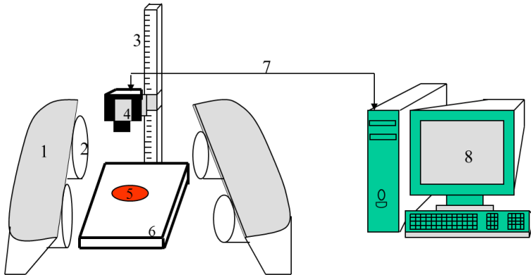
1 - Cover; 2- Lamp; 3 - Stand ; 4- Camera; 5 - Apple fruit ample; 6- Stand basis; 7 -Electric wire; and 8- Personal computer.
