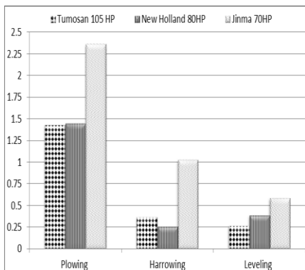
Fig.(7) Slip horsepower (kW) Interaction between tractors and oper.
