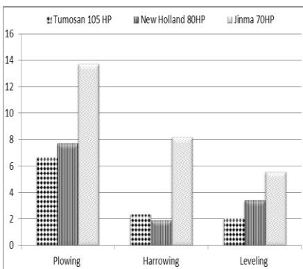
Fig.(6) Slip percentage (%) Interaction between tractors and operation
