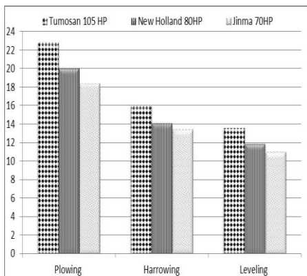
Fig.(9) Total engine horsepower required (kW) Inter. between tractors and oper.
