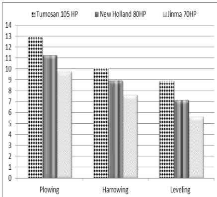
Fig. (4) Drawbar pull horsepower (kW) Inter. between tractors % oper.
