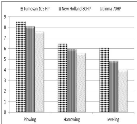
Fig. (3) Net drawbar pull (kN) Inter. between tractors and operation.
