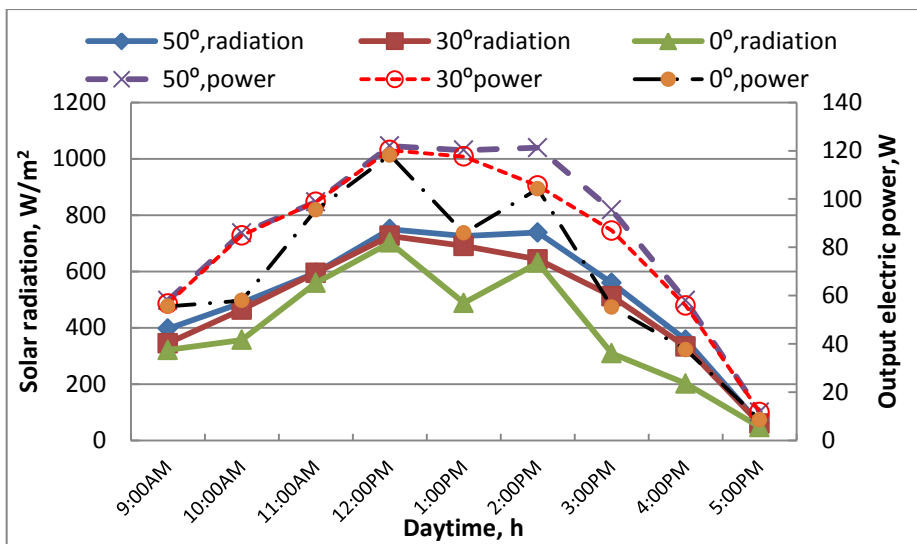
Figure 7. Effect of daytime on solar radiation and output electric power at different tilt angles ( 0^{\circ} , 30^{\circ} and 50^{\circ} ) and fixed system toward south and sun tracking from east to west throughout the courses of days in winter, 2011.
