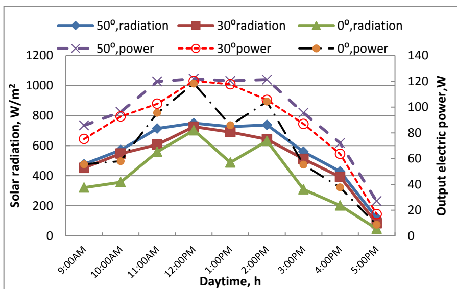
Figure 7. Effect of daytime on solar radiation and output electric power at different tilt angles ( 0^{\circ} , 30^{\circ} and 50^{\circ} ) and fixed system toward south and sun tracking from east to west throughout the courses of days in winter, 2011.
