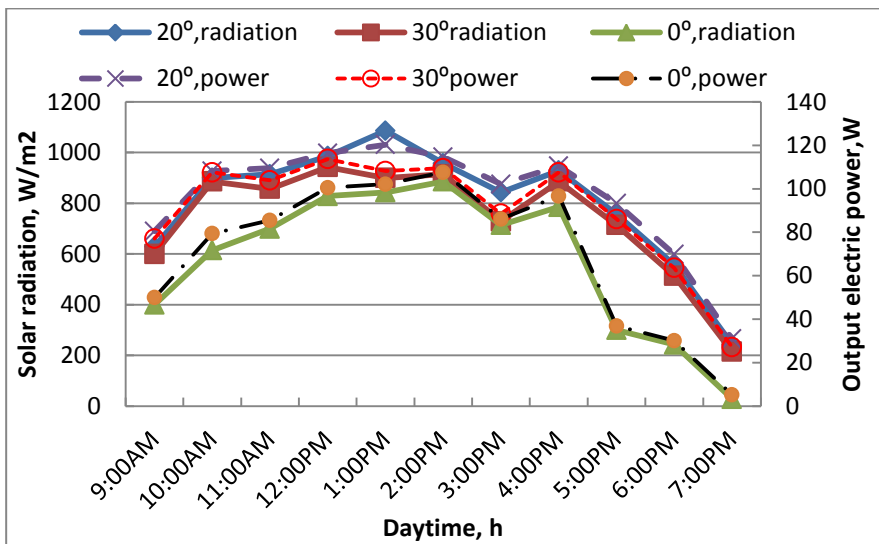
Figure 6. Effect of daytime on solar radiation and output electric power at different tilt angles ( 0^{\circ} , 20^{\circ} and 30^{\circ} ) and moved system by sun tracking device from east to west throughout the courses of days in summer, 2010
