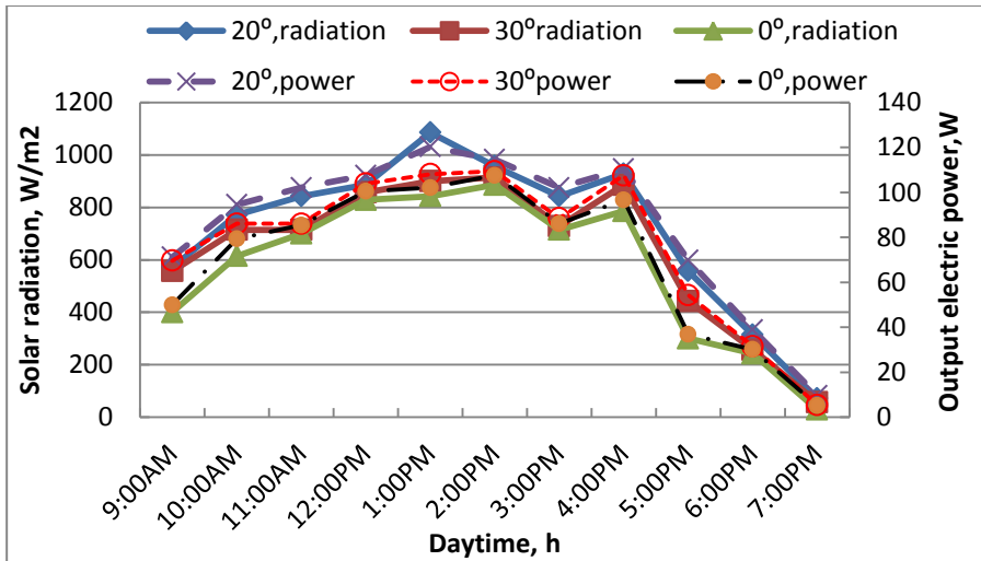
Figure 5. Effect of daytime on solar radiation and output electric power at different tilt angles ( 0^{\circ} , 20^{\circ} and 30^{\circ} ) and fixed system toward south and sun tracking from east to west throughout the courses of days in summer, 2010.
