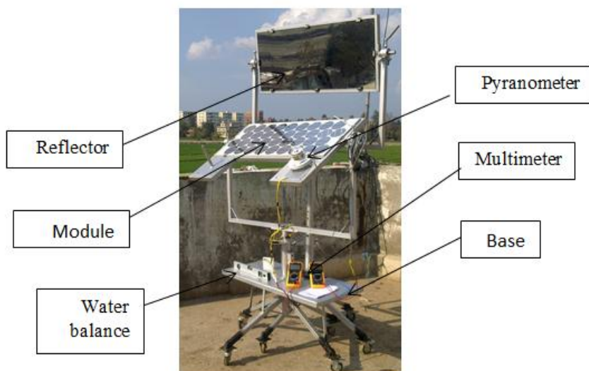
Figure 2. Photograph of reflector with module
