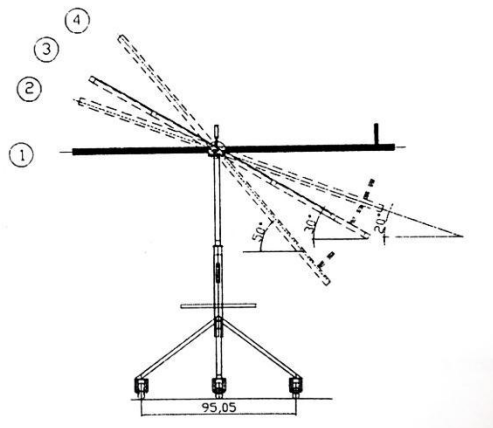
Figure 3. Setup for tilt angle test.
